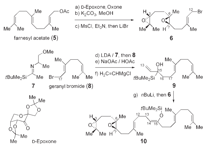
Scheme 2. Synthesis of squalene-like substrate 10 for biomimetic cyclizations. Reagents and conditions: a) D-Epoxone (0.5 equiv), Oxone, pH 10.5 buffer, DMM/MeCN/H 2 O, -5^\circ\text{C} , 54%; b) K 2 CO 3 , MeOH, 99%; c) MsCl, Et 3 N, -40^\circ\text{C} , then LiBr, THF, 0^\circ\text{C} , 60%; d) LDA, THF, -30^\circ\text{C} , then 8 ; e) NaOAc, HOAc, 84% (2 steps); f) H 2 C=CHMgCl, Et 2 O, 0^\circ\text{C} , then HCl, 88%; g) n BuLi, hexane/THF, -78^\circ\text{C} , then 6 , 50%. DMM = dimethoxymethane.
