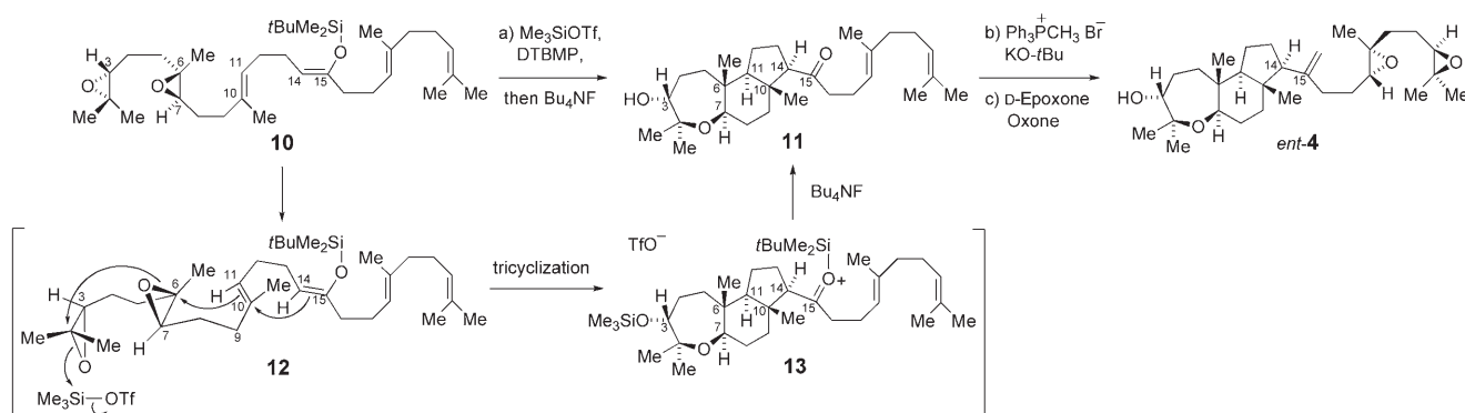
Scheme 3. Biomimetic tricyclization of 10 to 11 , and conversion into ent - 4 . Reagents and conditions: a) Me 3 SiOTf, DTBMP, CH 2 Cl 2 , -78^\circ\text{C} , then Bu 4 NF, 50%; b) Ph 3 PMeBr, KO- t Bu, benzene, 80^\circ\text{C} , 30% (+ 55% C14 epimer); c) D-Epoxone (0.5 equiv), Oxone, pH 10.5 buffer, DMM/MeCN/H 2 O, -5^\circ\text{C} , 50%.
